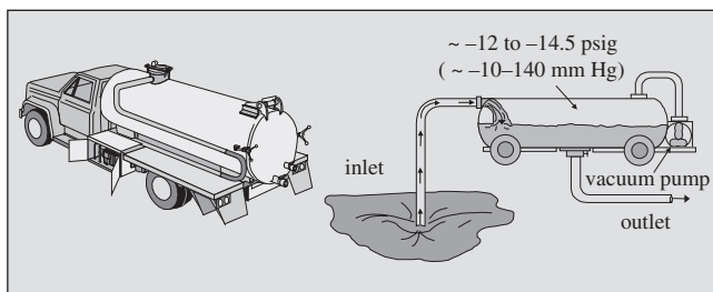
Figure 11-13 Vacuum Truck
