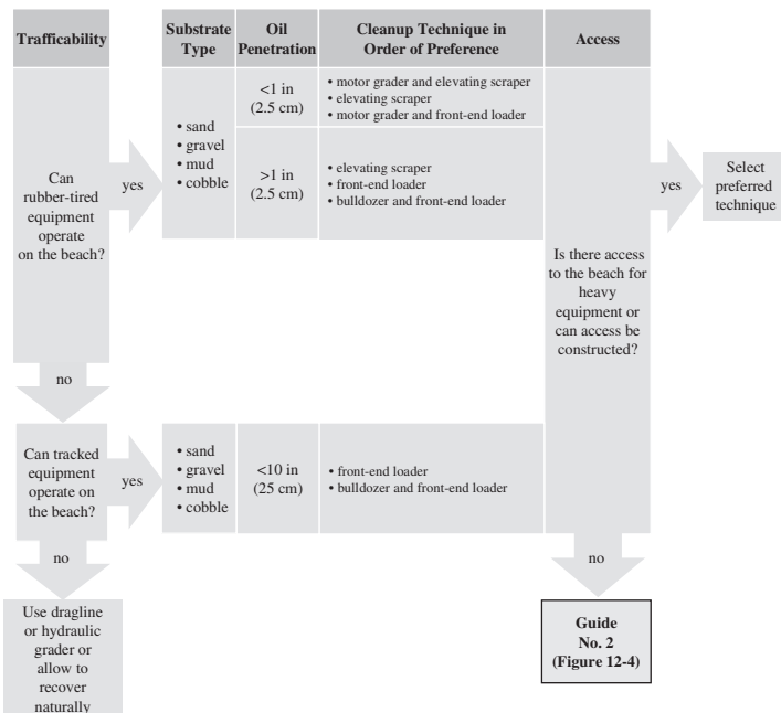
Figure 12-3 Shoreline Treatment Guide No. 1
