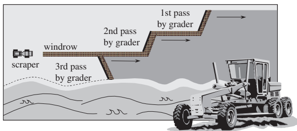
Figure 12-15 Motor Grader/Elevating Scraper Combination Treatment Pattern
