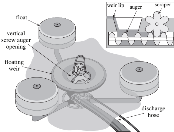
Figure 9-5 Weir with Integral Screw Auger
