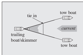
Figure 5-13 V-Booming
