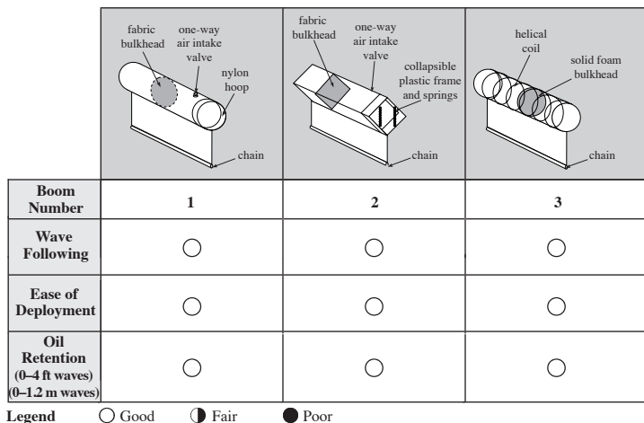
Figure 5-8 Self-Inflating Boom
