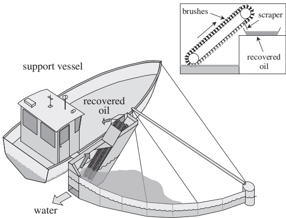
Figure 9-16 Brush Skimmer
