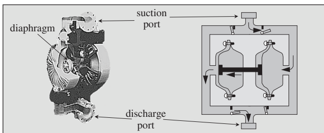
Figure 11-10 Diaphragm Pump
