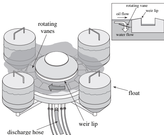
Figure 9-19 Rotating Vane Skimmer
