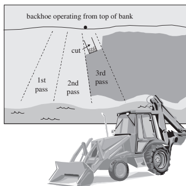
Figure 12-19 Backhoe with Front Bucket Treatment Pattern
