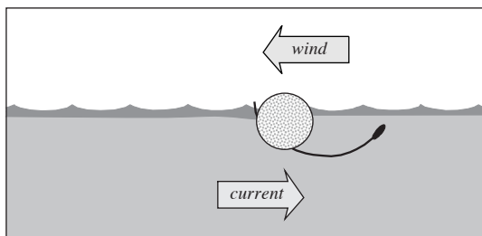
Figure 5-6 Planing Failure
