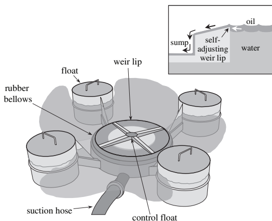
Figure 9-3 Self-Leveling Weir
