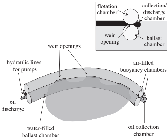
Figure 9-7 Weir Boom Skimmer
