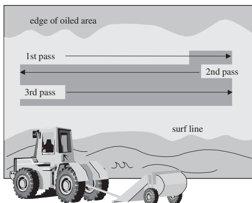
Figure 12-10 Beach Cleaner Treatment Pattern
