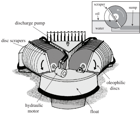
Figure 9-10 Disc Skimmer
