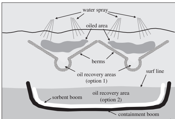
Figure 12-6 Low Pressure Flushing
