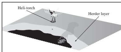
Figure 8-3 Conceptual drawing showing a helicopter herder – ISB system
