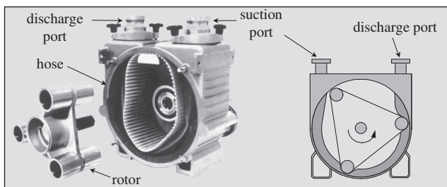
Figure 11-11 Peristaltic Pump
