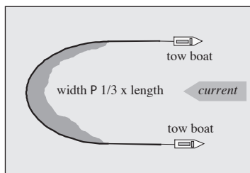
Figure 5-12 U-Booming
