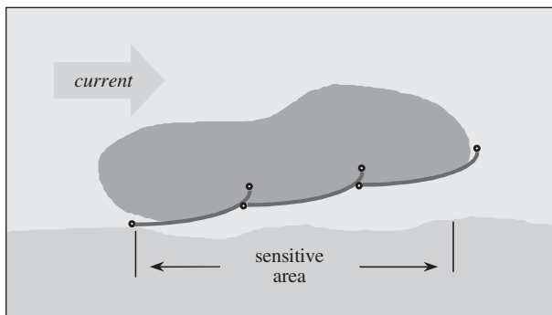
Figure 6-2 Diversion Booming
