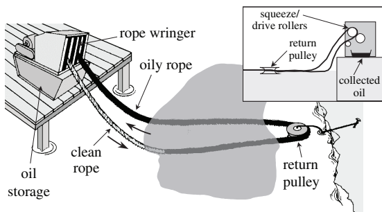
Figure 9-12 Horizontal Rope Mop Skimmer
