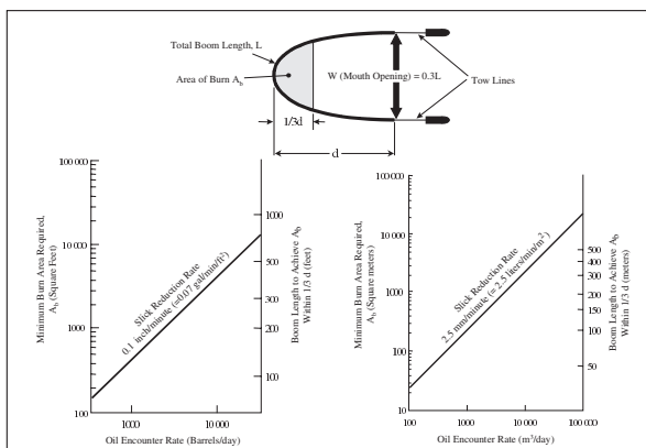
Figure 8-2 Estimating Area Required for Various Oil Encounter Rates
