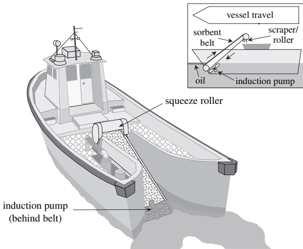
Figure 9-15 Sorbent Lifting Belt
