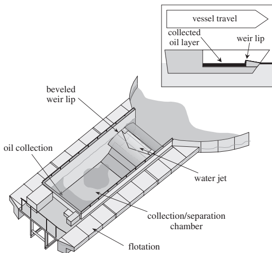
Figure 9-6 Advancing Weir Skimmer
