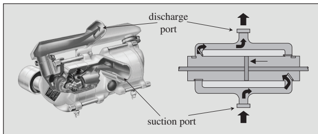
Figure 11-9 Reciprocating Pump
