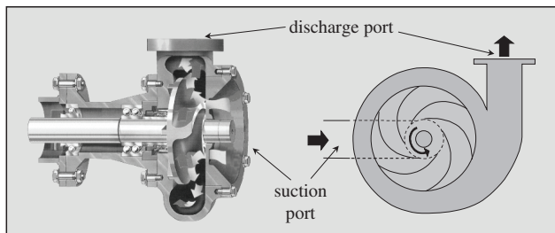
Figure 11-1 Centrifugal Pump
