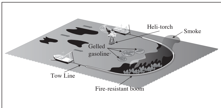
Figure 16-4 In-Situ Burn Operation using a helicopter and heli-torch
