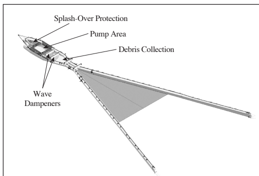
Figure 5-16 General Current Buster® Configuration
