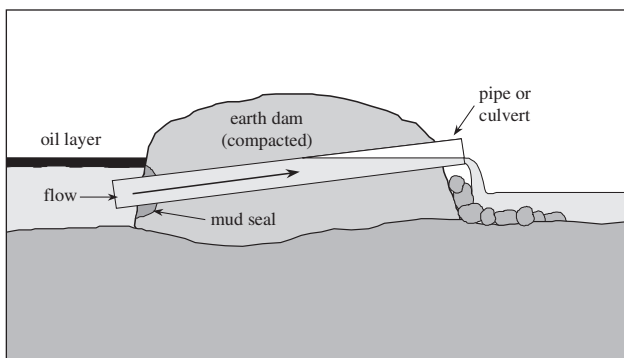
Figure 6-6 Inverted Weir
