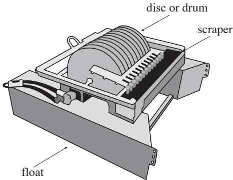
Figure 9-11 Fabric-Coated Disc Skimmer
