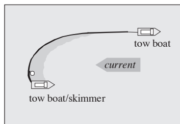
Figure 5-14 J-Booming
