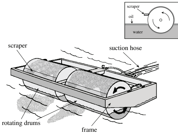
Figure 9-8 Drum Skimmer
