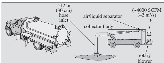
Figure 11-14 Air Conveyor
