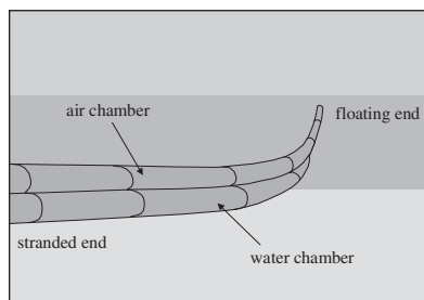
Figure 6-4 Shore-Sealing Boom
