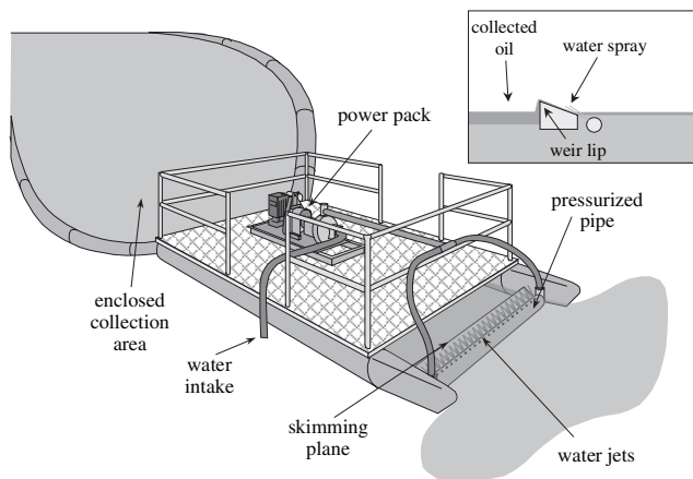
Figure 9-17 Water Jet Skimmer
