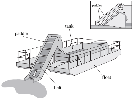
Figure 9-20 Paddle Belt Skimmer
