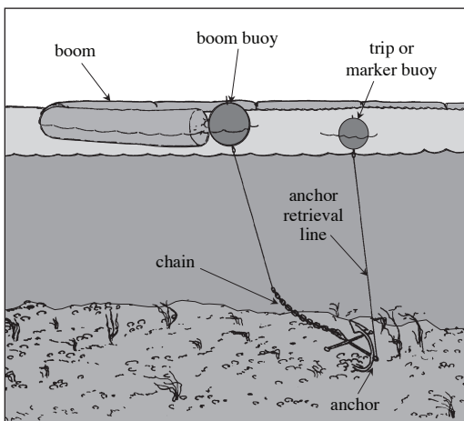
Figure 5-17 Boom Anchoring Assembly
