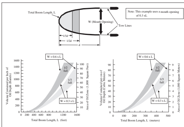
Figure 8-1 Estimating Boom Holding Capacity
