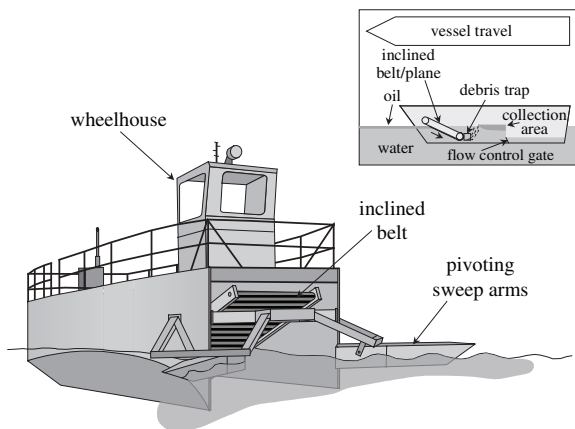
Figure 9-18 Submersion Plane/Belt Skimmer
