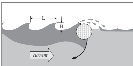
Figure 5-4 Splashover Failure
