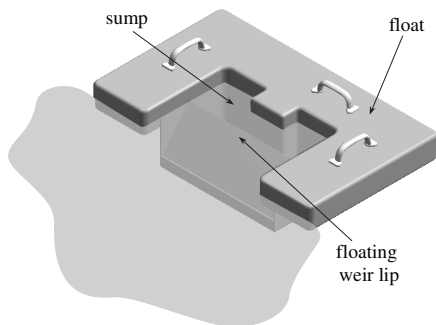
Figure 9-4 Self-Leveling Weir
