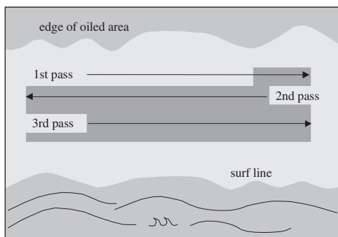
Figure 12-11 Tractor/Ripper Treatment Pattern
