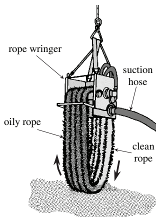
Figure 9-13 Vertical Rope Mop Skimmer
