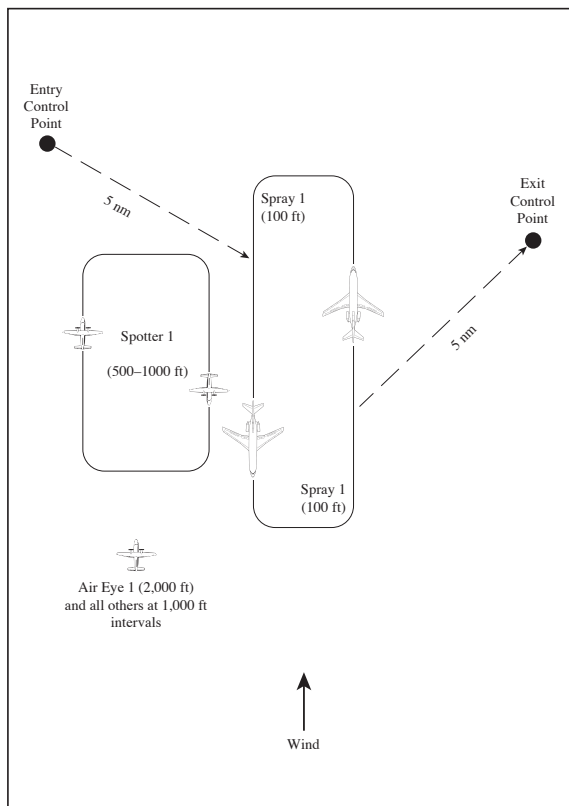
Figure 16-3 Diagram of Possible Dispersant Spray Operations to illustrate coordination and scheduling of aircraft movements and operations
