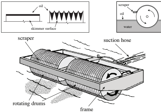
Figure 9-9 Grooved Drum Skimmer
