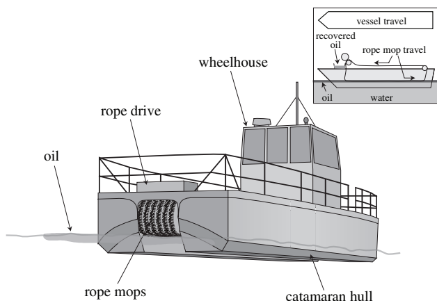
Figure 9-14 ZRV Rope Mop Skimmer
