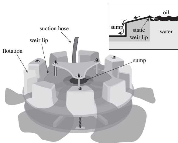
Figure 9-2 Simple Weir Skimmer
