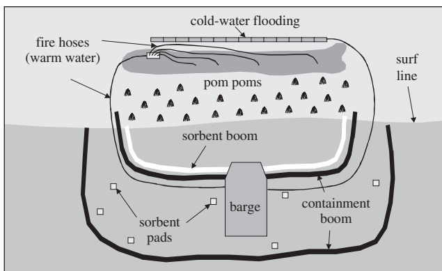
Figure 12-7 Low-Pressure, Warm-Water Washing/Cold-Water Flooding
